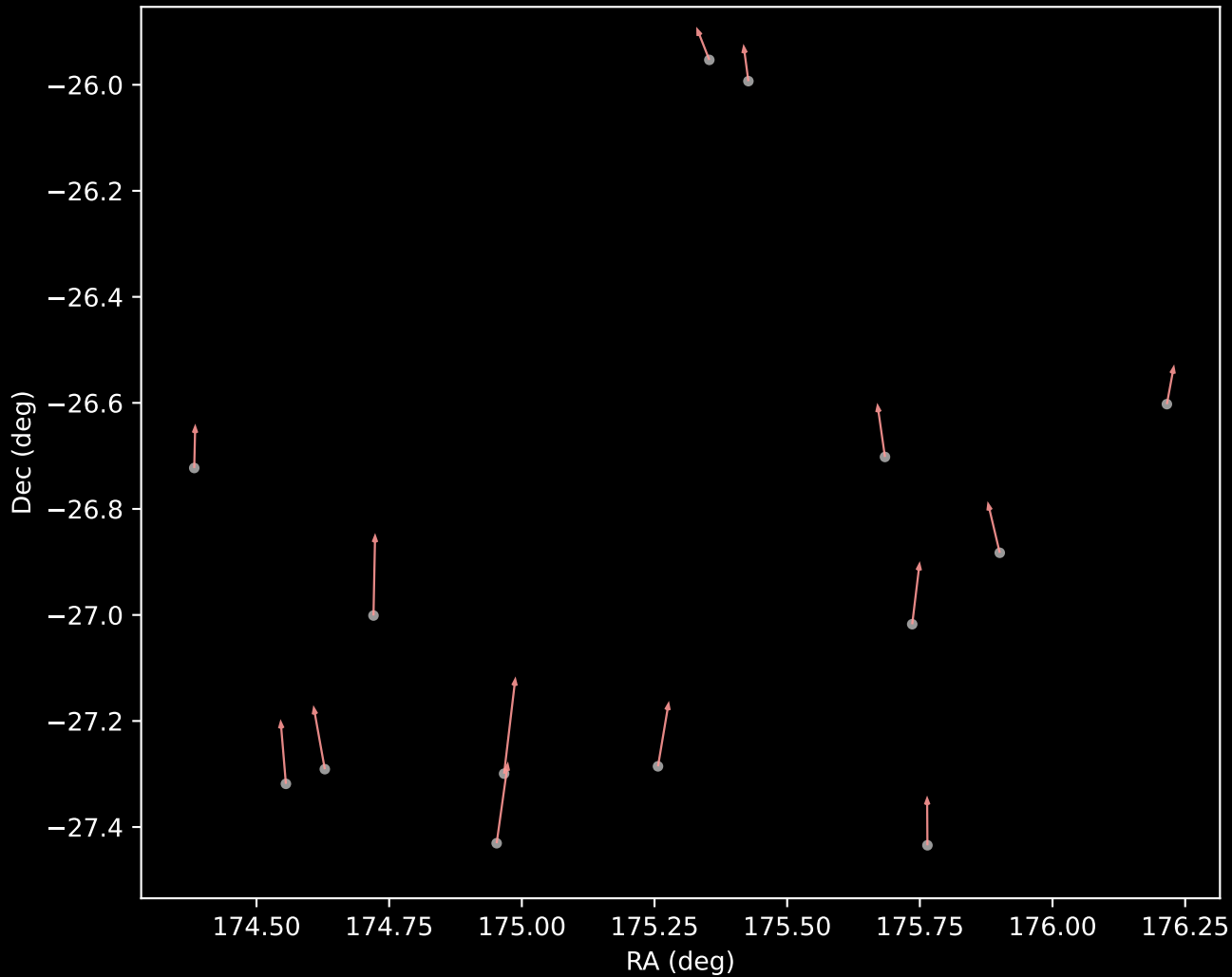
GALAH DR4 Cluster 7 Proper Motion Vectors (n=14)
