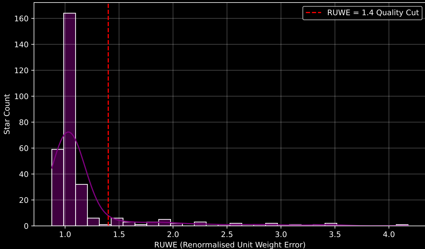
GALAH DR4 Field [556] RUWE Distribution (n= 296)
