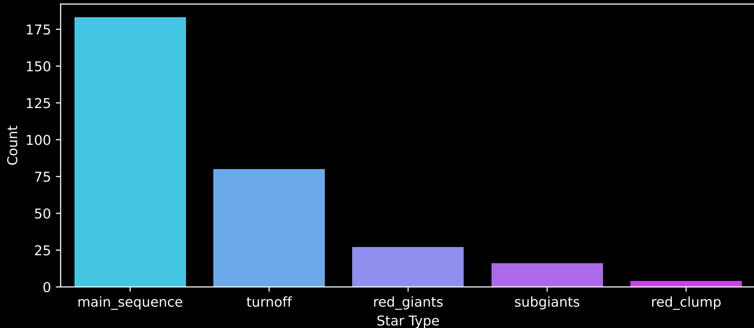
GALAH DR4 Field: [556] Count plot of Star Type
