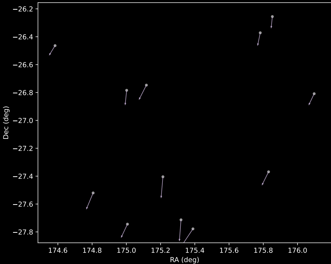
GALAH DR4 Cluster 9 Proper Motion Vectors (n=12)
