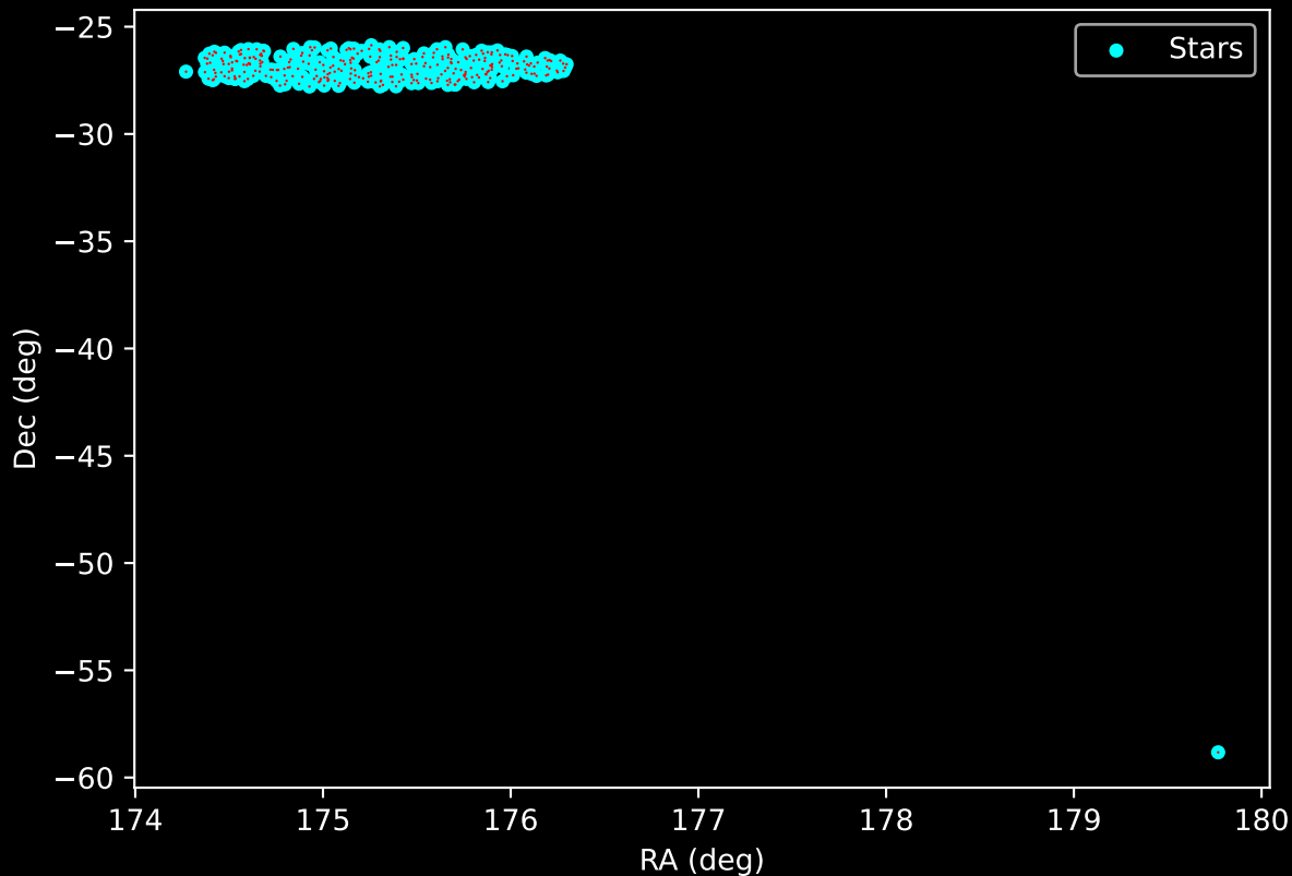
GALAH DR4 Field: [556] Proper Motion Vectors for Gaia Star Field (n= 310)
