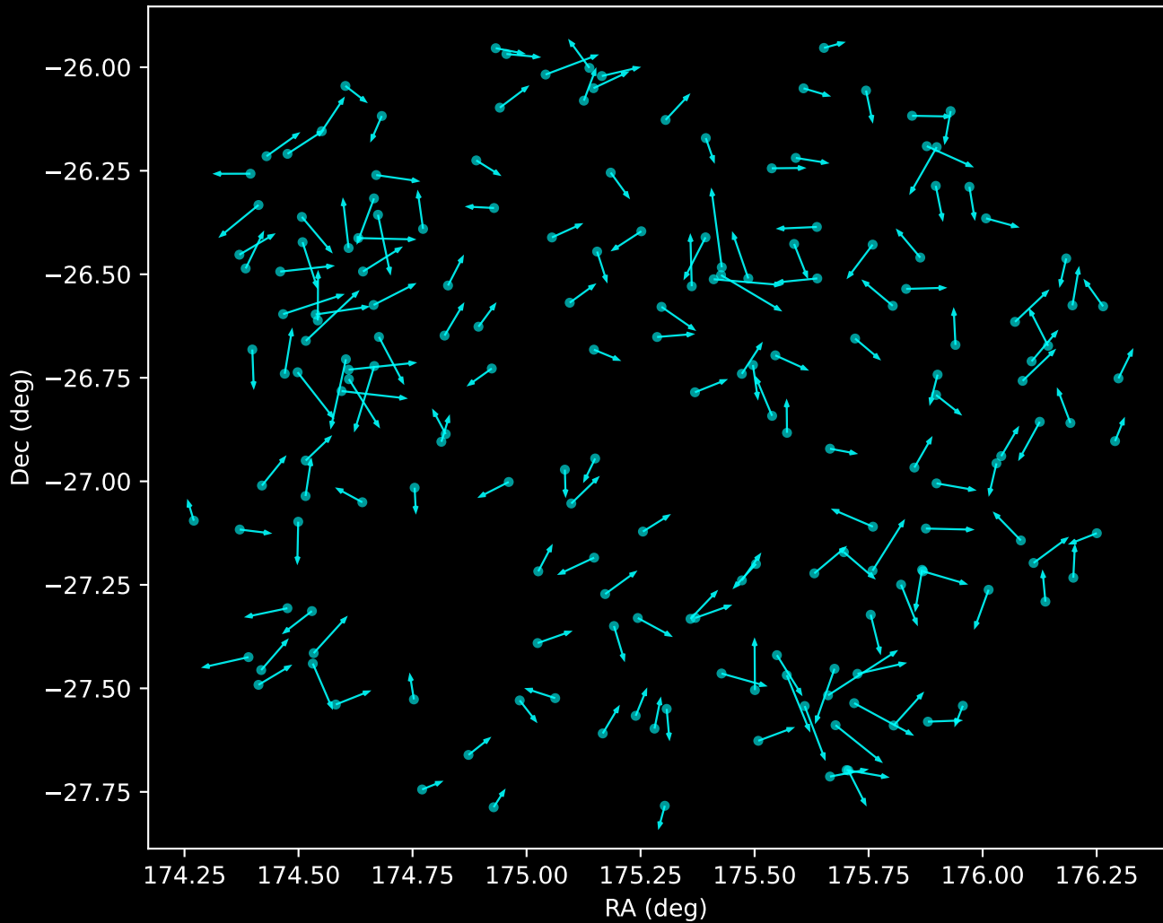
GALAH DR4 Noise Stream Proper Motion Vectors (n=184)
