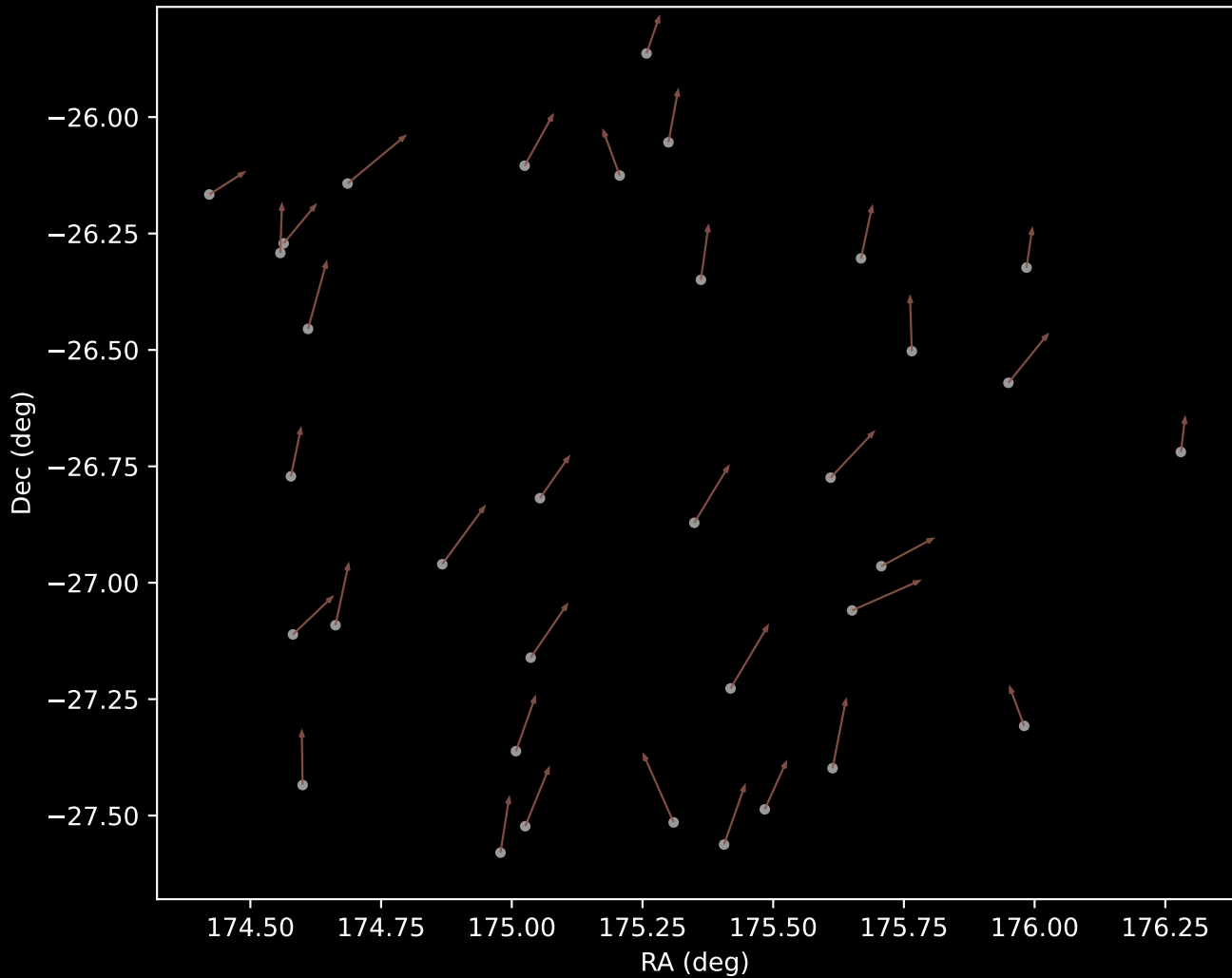
GALAH DR4 Cluster 10 Proper Motion Vectors (n=35)
