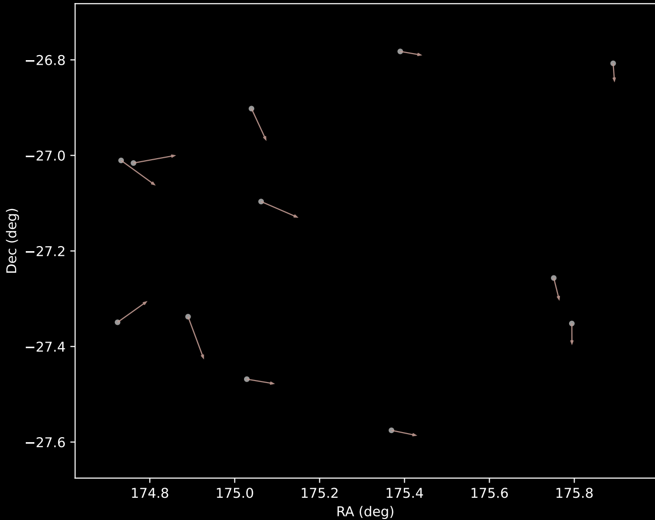
GALAH DR4 Cluster 11 Proper Motion Vectors (n=12)
